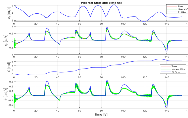
Figure 3.3: State estimation: comparison between the true state, the proposed NAO, and the PI observer (without loss accumulation).
