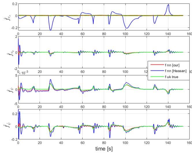
Figure 3.5: Unknown-input estimation: comparison of the proposed NAO against the baseline approach of [GHANI20235685].
