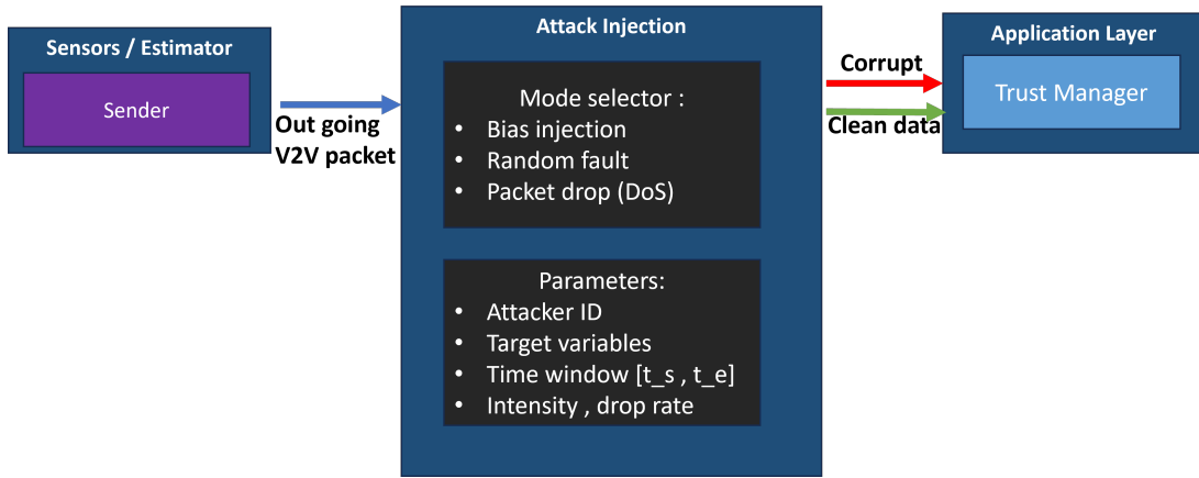
Figure 5.5: Attack injection mechanism integrated into the V2V communication layer.
