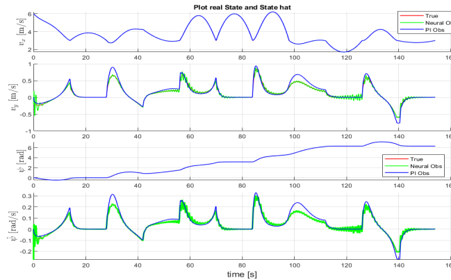
Figure 3.3: State estimation: comparison between the true state, the proposed NAO, and the PI observer (without loss accumulation).
