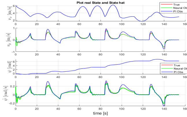
Figure 3.4: State estimation with loss accumulation. The accumulation mitigates transient spikes and reduces estimation noise.
