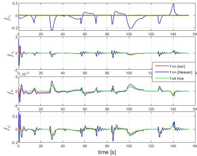
Figure 3.5: Unknown-input estimation: comparison of the proposed NAO against the baseline approach of [23].
