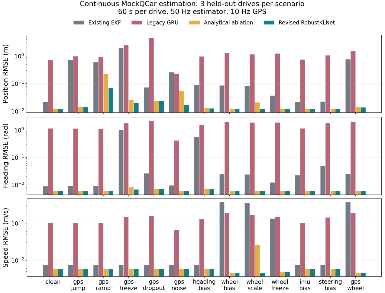
Figure 1: Continuous held-out estimation. Logarithmic axes preserve both clean accuracy and large attack errors. The analytical ablation separates the learned trust contribution from the new physical predictor and guards.
