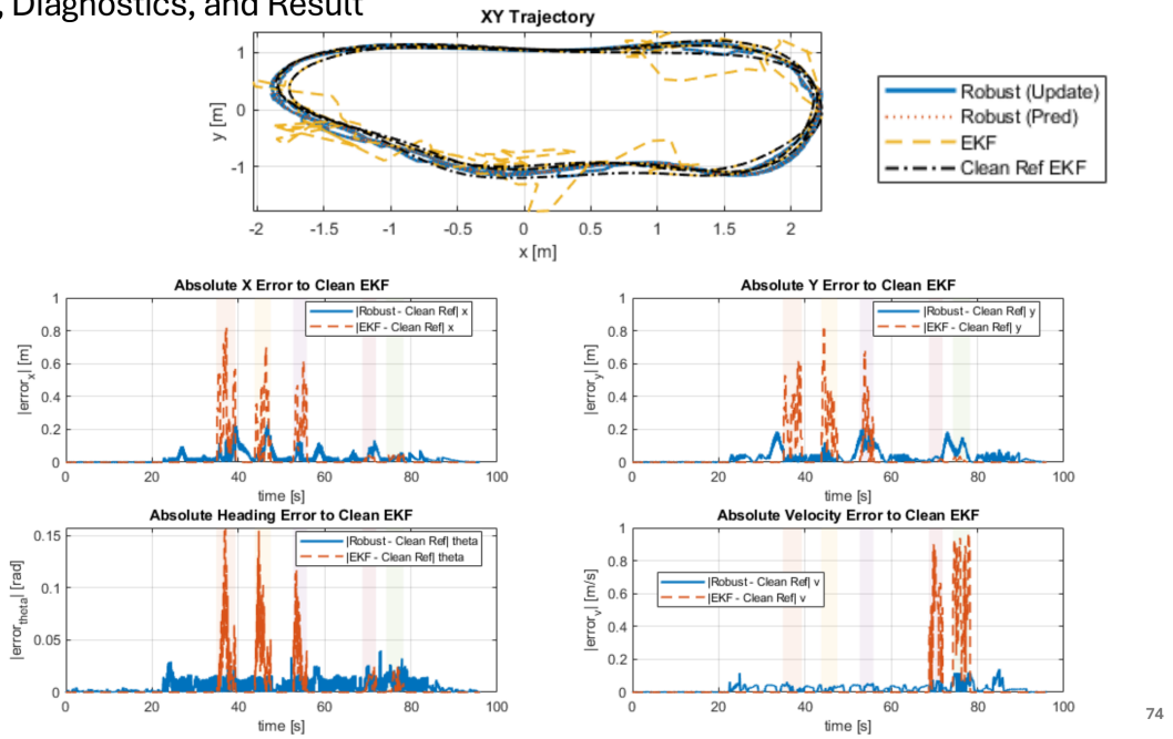
Figure 4: State-estimation behavior during the runtime comparison. The robust estimator follows the clean-reference EKF while the ordinary EKF shows larger spikes during attack intervals.
