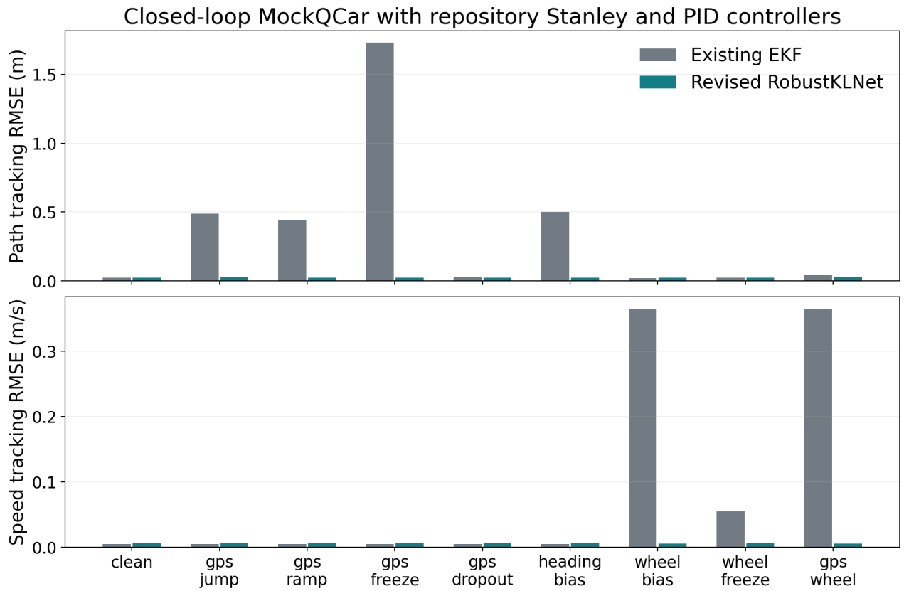
Figure 2: Closed-loop path and speed error after the initial 3 s startup period. The EKF and revised estimator drive separate plant trajectories.
