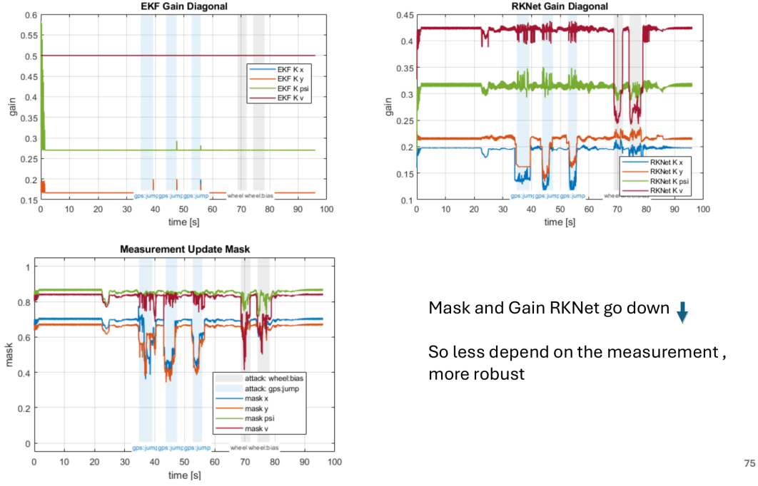
Figure 5: Gain and measurement-mask behavior during the runtime comparison. The learned mask and effective gain decrease during GPS jump and wheel-bias intervals, reducing dependence on corrupted measurements.
