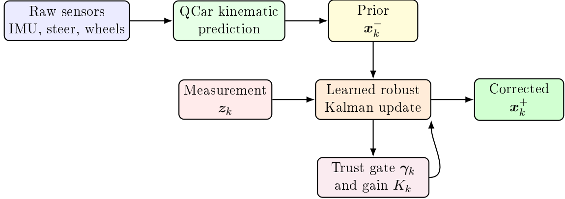
Figure 3: Hybrid RKNet structure used in this work. The prior is generated by QCar physics. The neural update learns a measurement trust gate and a Kalman-style gain.
