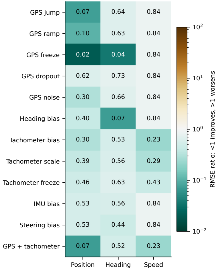
First 3 s after removal: hybrid / EKF
