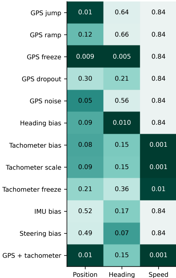
During injection: hybrid / EKF
