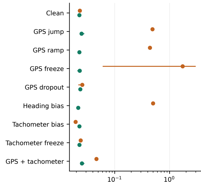
(a) Closed-loop path RMSE (m)
