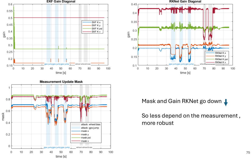
Figure 3: Gain and measurement-mask behavior during the runtime comparison. The learned mask and effective gain decrease during GPS jump and wheel-bias intervals, reducing dependence on corrupted measurements.
