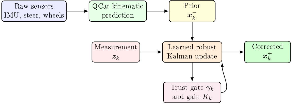
Figure 1: Hybrid RKNNet structure used in this work. The prior is generated by QCar physics. The neural update learns a measurement trust gate and a Kalman-style gain.
