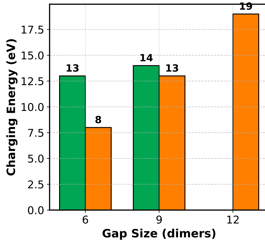
Charging Energy (eV)
