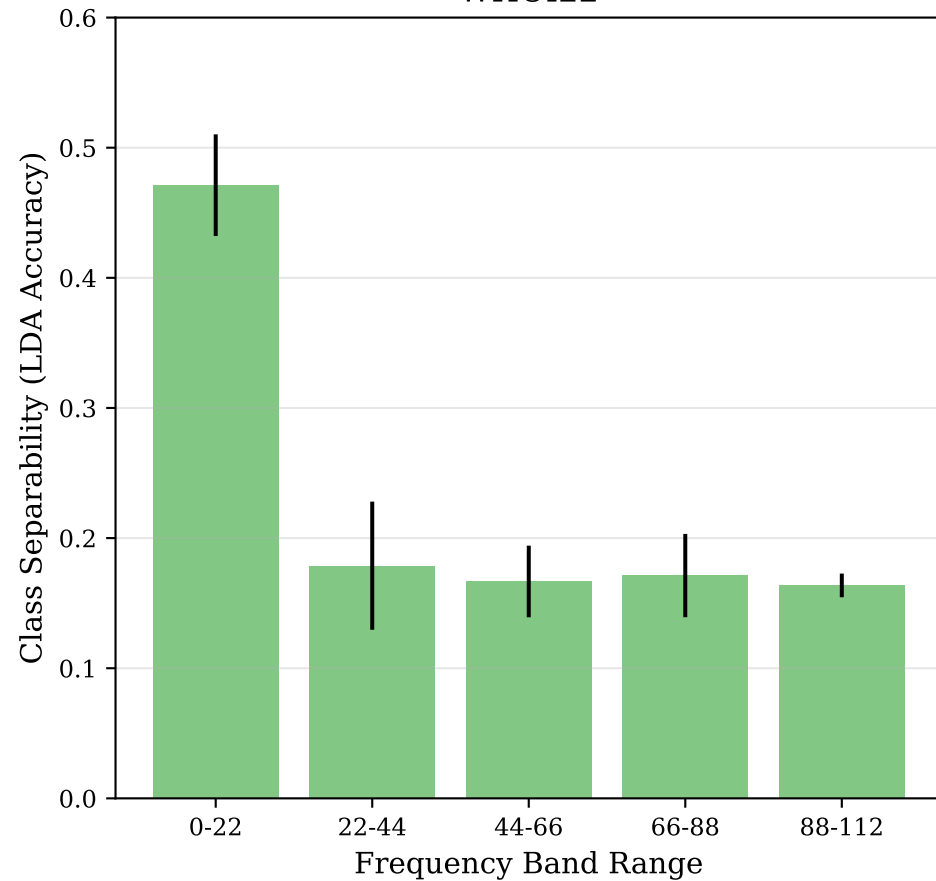
WHOI22
