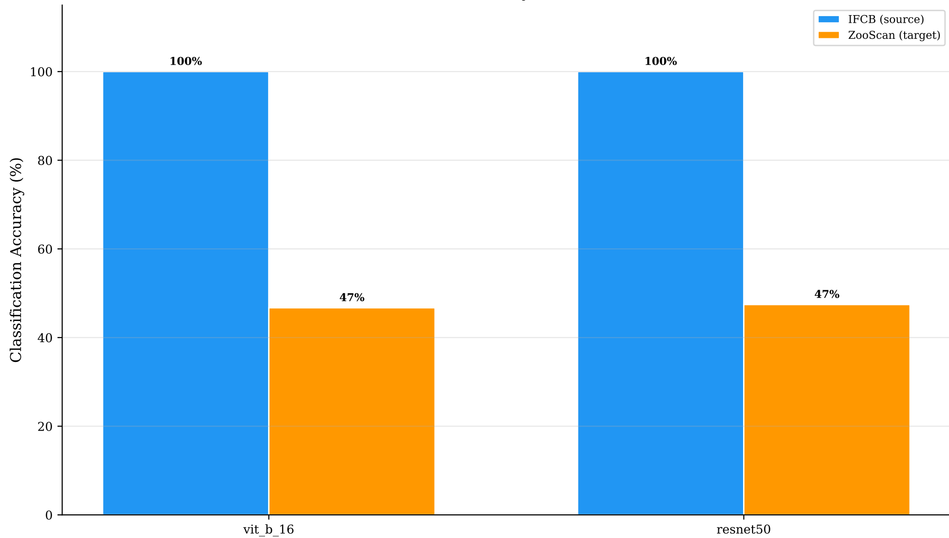
Cross-Domain Accuracy: IFCB \rightarrow ZooScan
