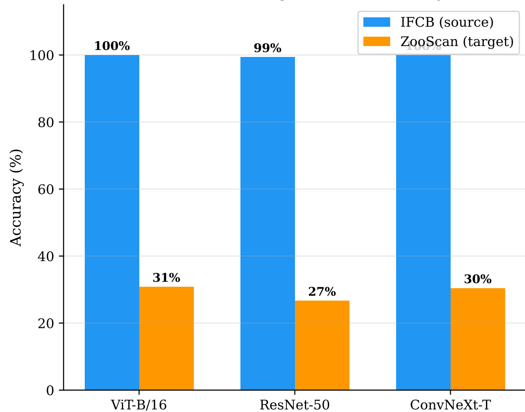
(a) Source vs target domain accuracy
