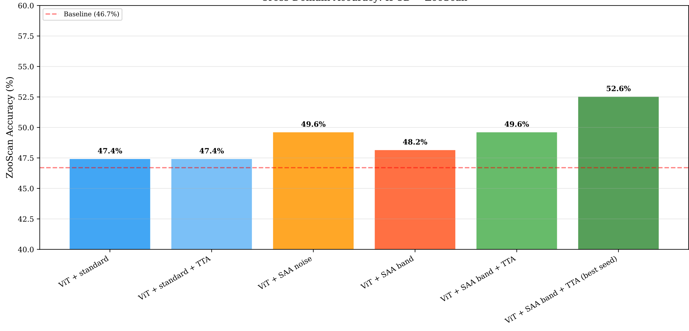
Cross-Domain Accuracy: IFCB \rightarrow ZooScan
