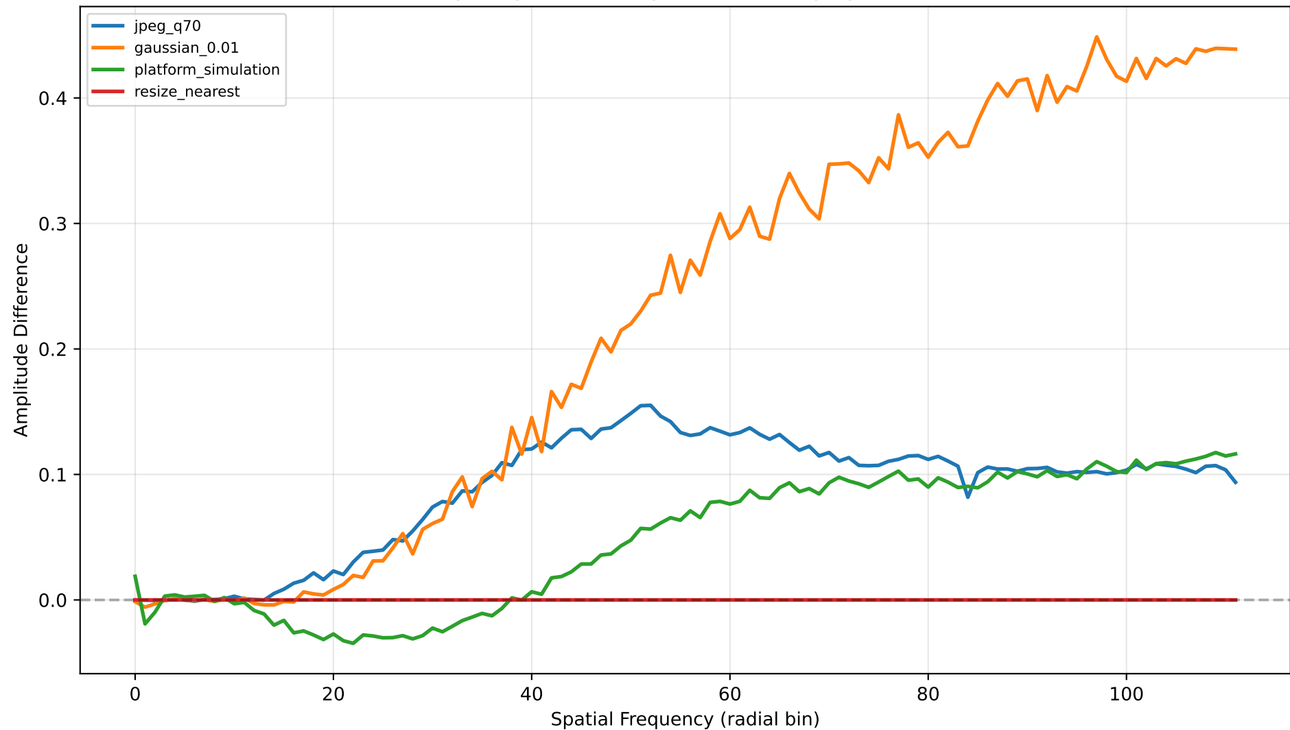
Frequency-Domain Signature of Imaging Artifacts
