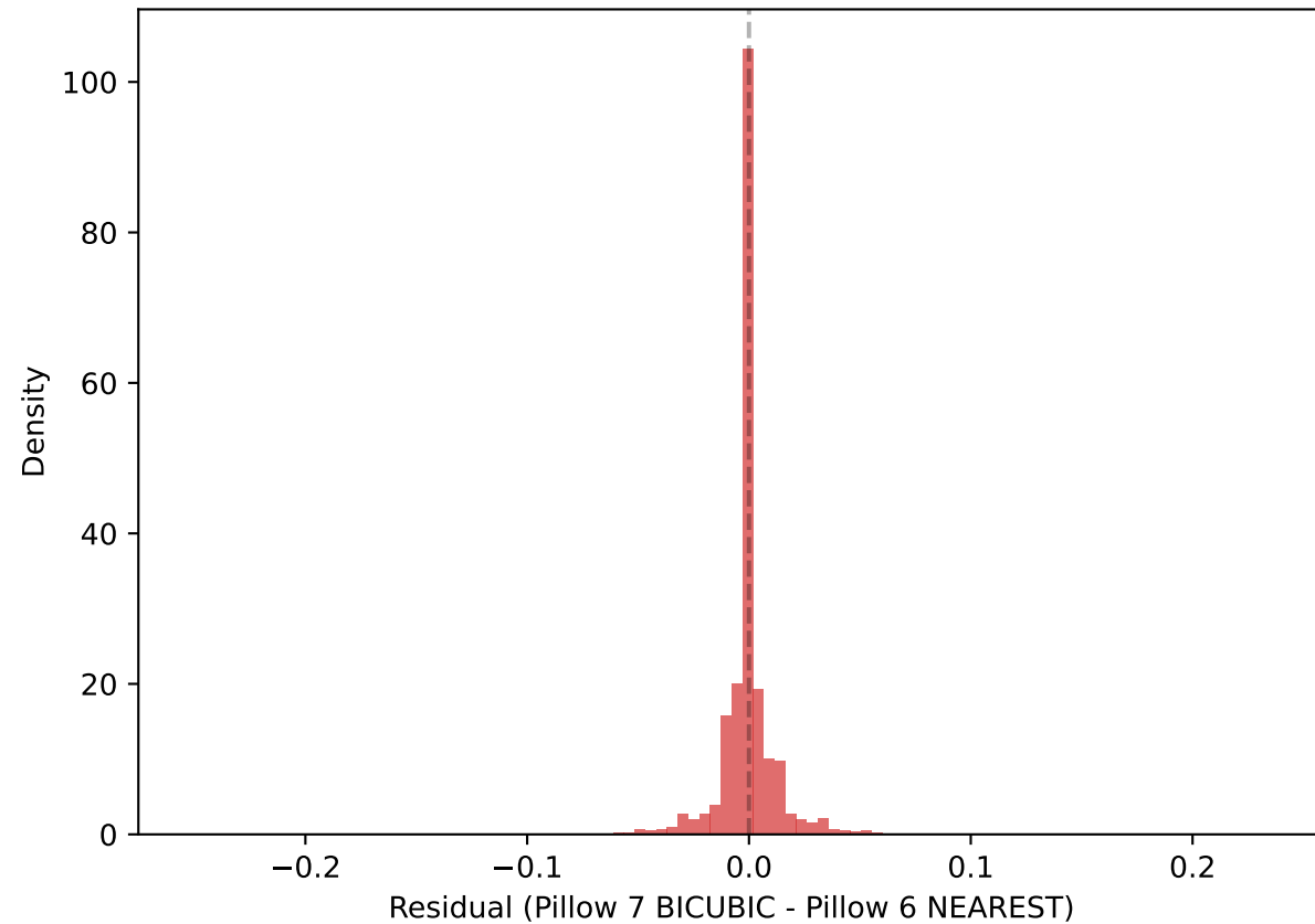
(a) Pixel residual distribution Pillow 6.2.2 vs 7.0.0 resize() default
