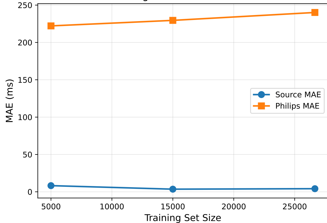
Scaling Law: Source vs OOD
