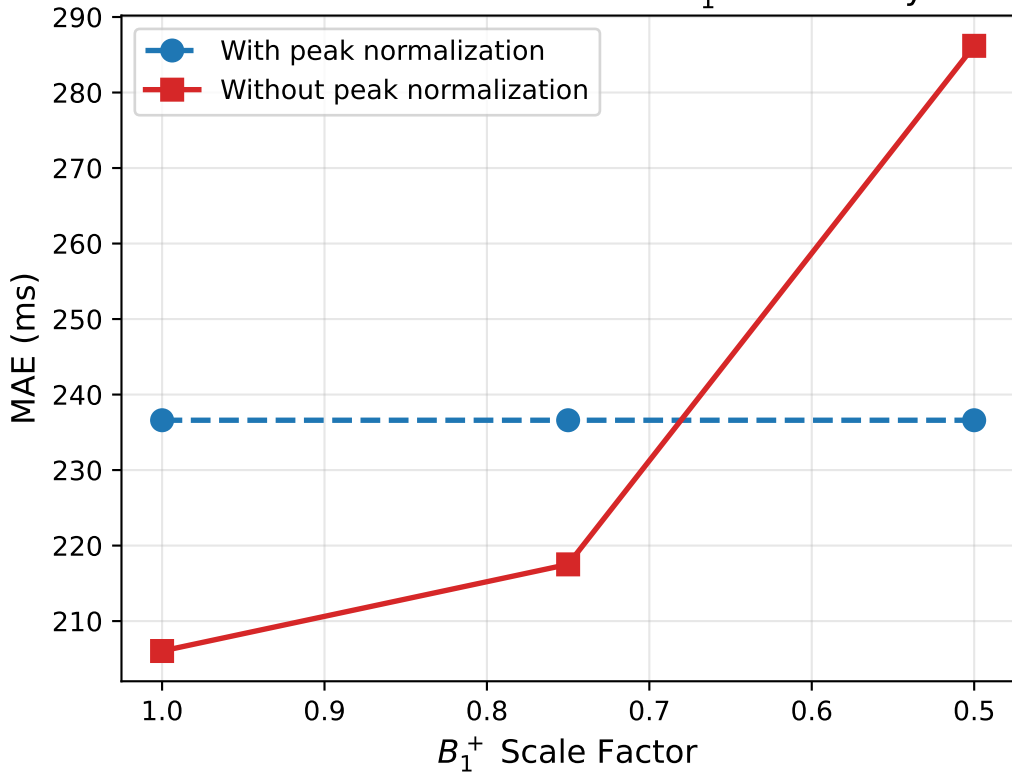
Peak Normalization Masks B_1^+ Sensitivity
