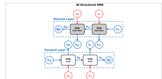
Bidirectional RNN
