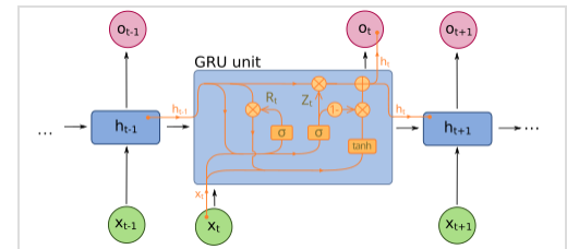
Gated recurrent unit
