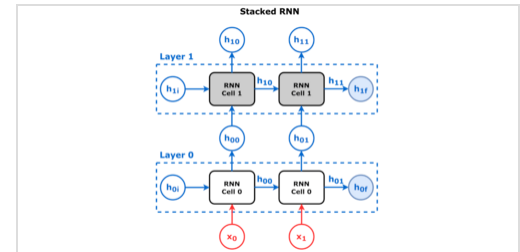
Stacked RNN
