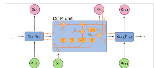
Long short-term memory unit
