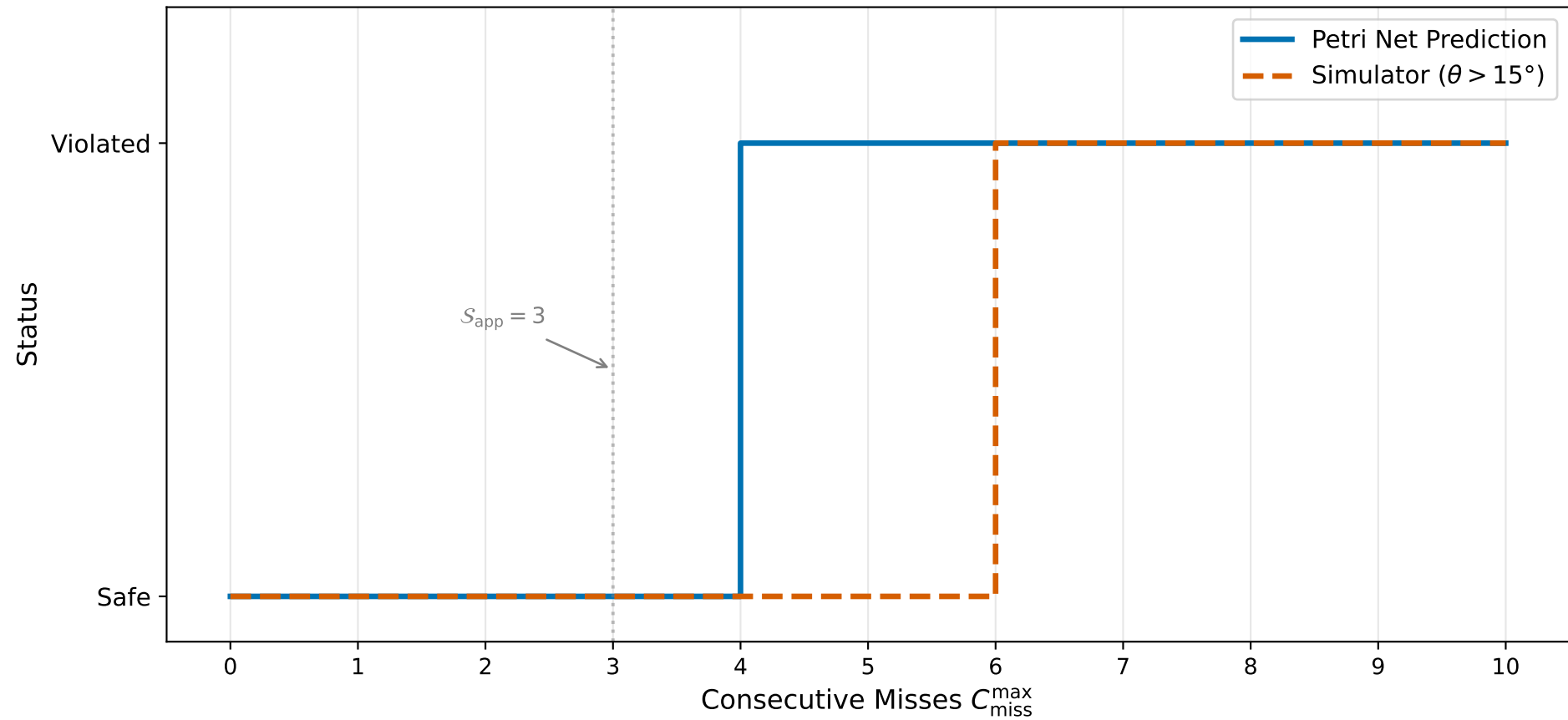
Petri Net Prediction vs. Simulator Angle Violation
