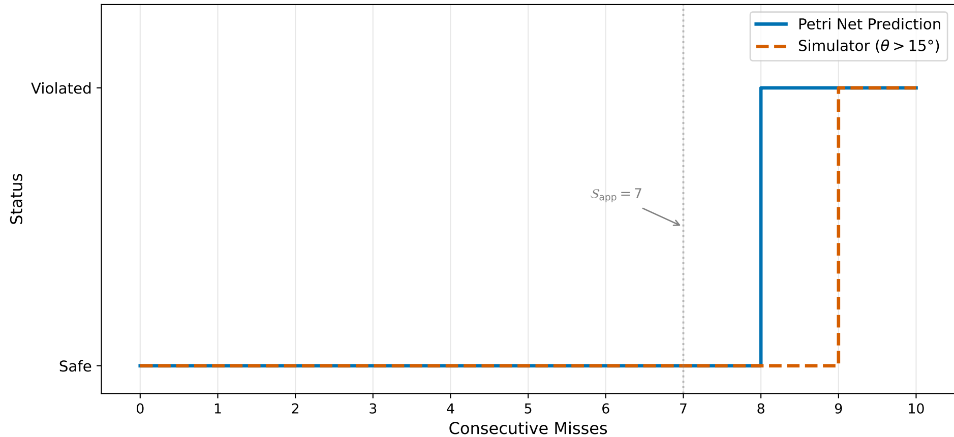
Petri Net vs.\ Simulator Angle Violation for mode \pi_1
