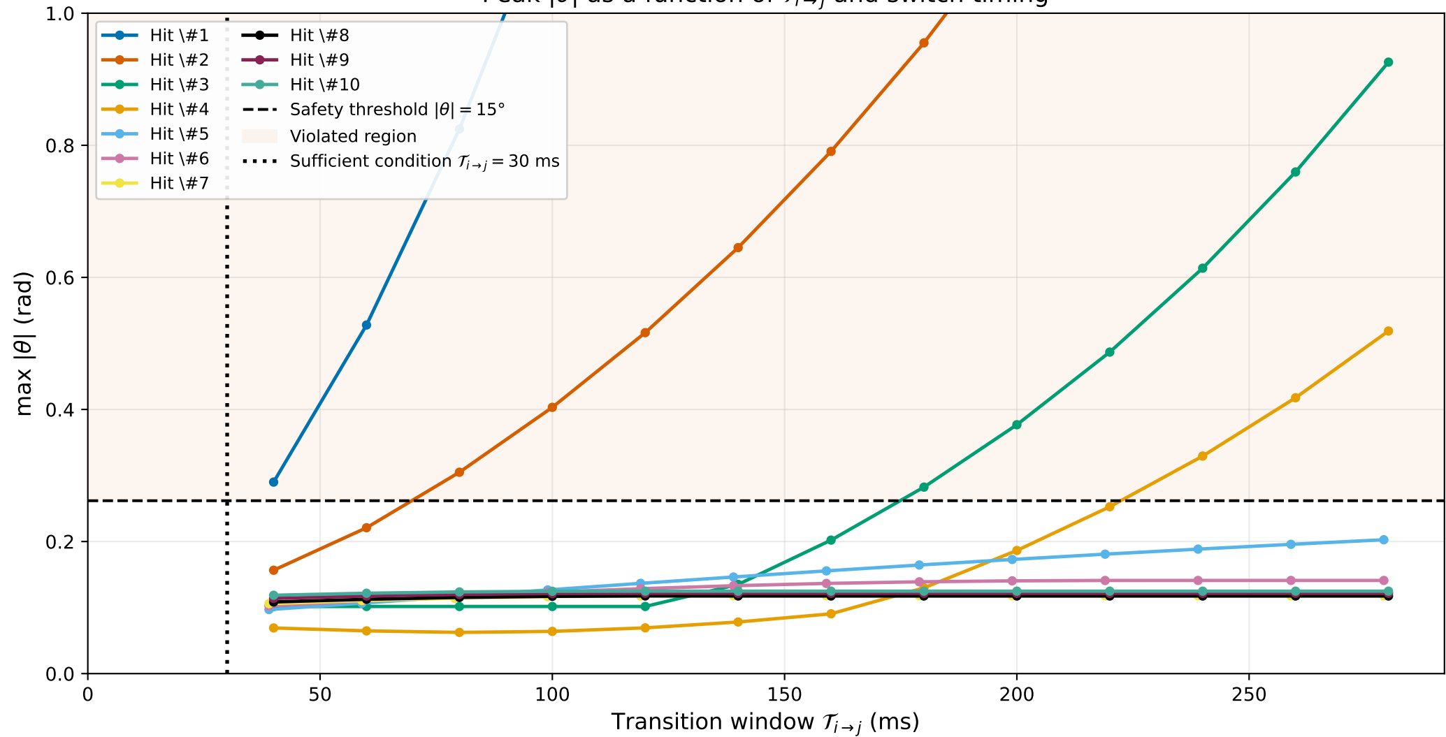
Peak |\theta| as a function of \tau_{i \rightarrow j} and switch timing
