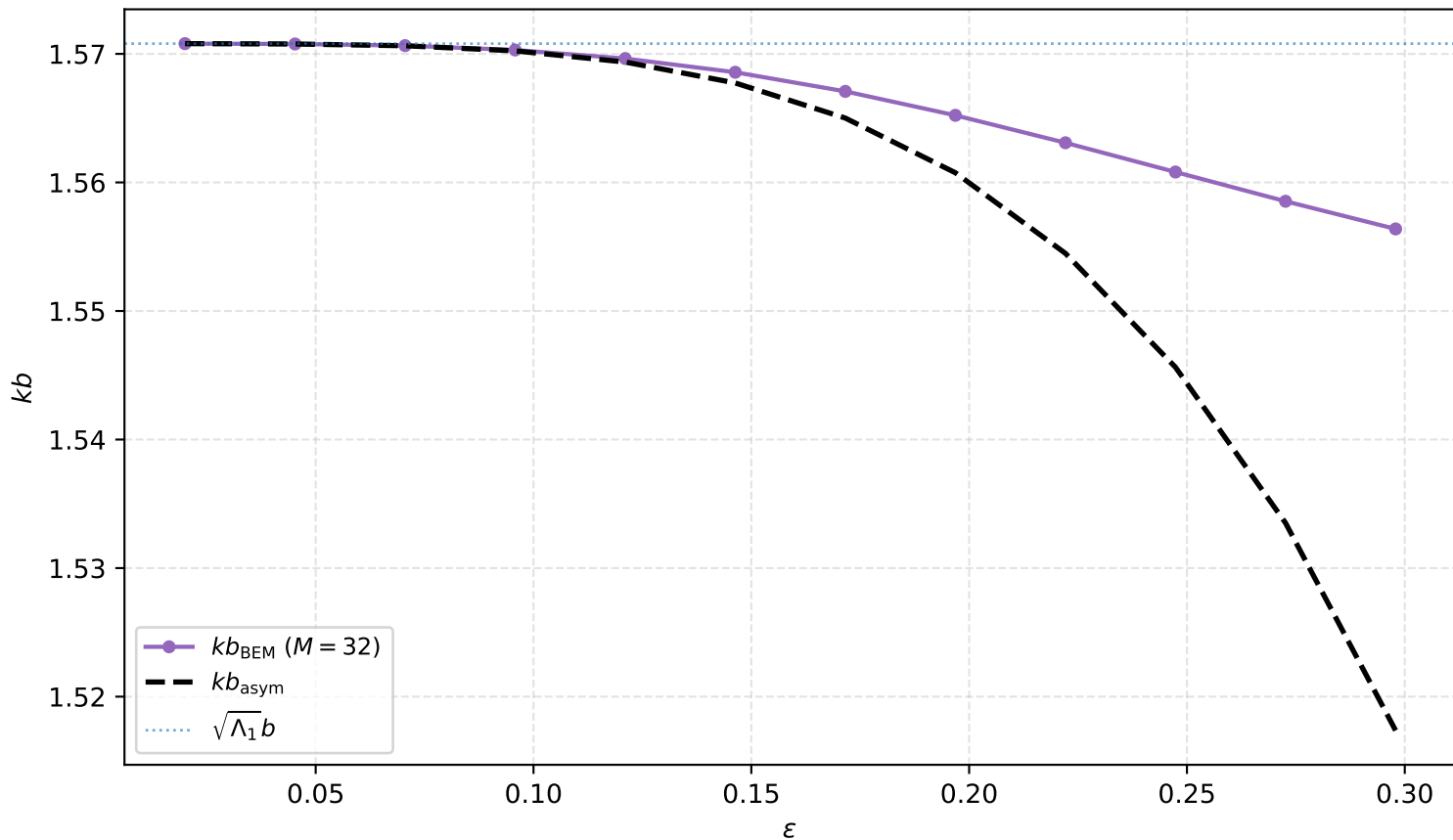
Theorem 2.1: kb versus \varepsilon , a = 0.65 , M = 32
