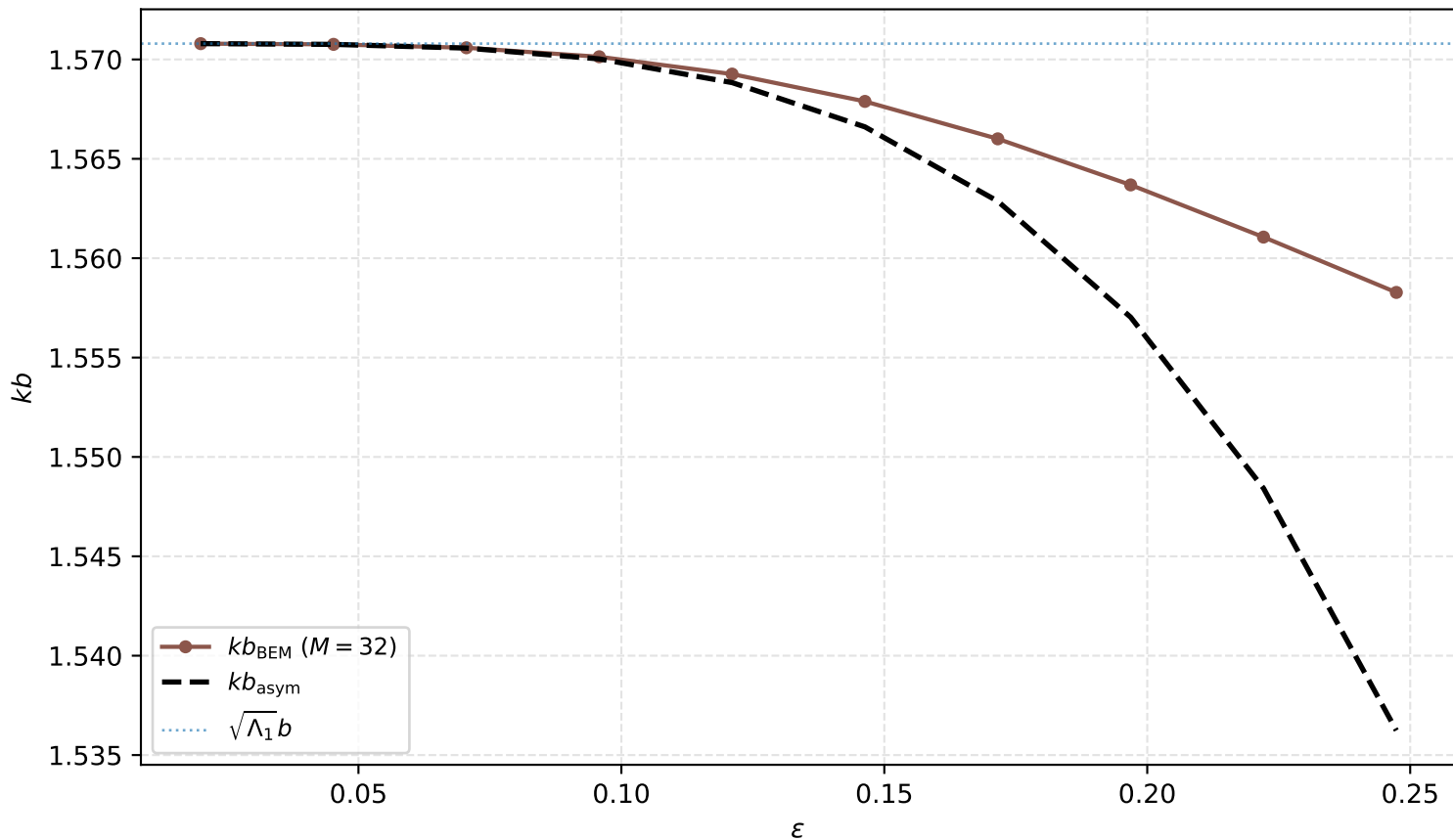
Theorem 2.1: kb versus \varepsilon , a = 0.70 , M = 32
