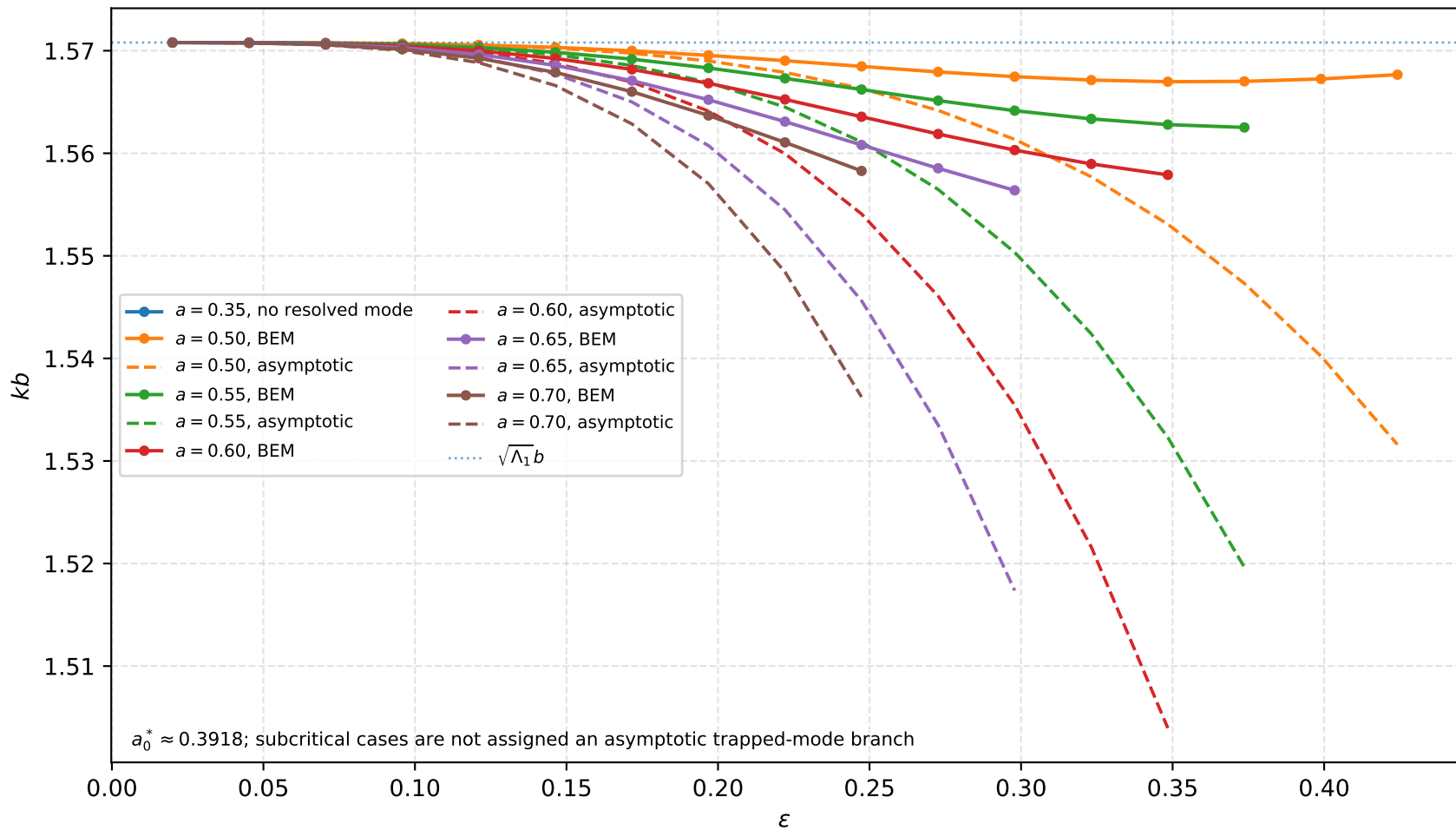
Theorem 2.1: dependence on obstacle height ( M = 32 )
