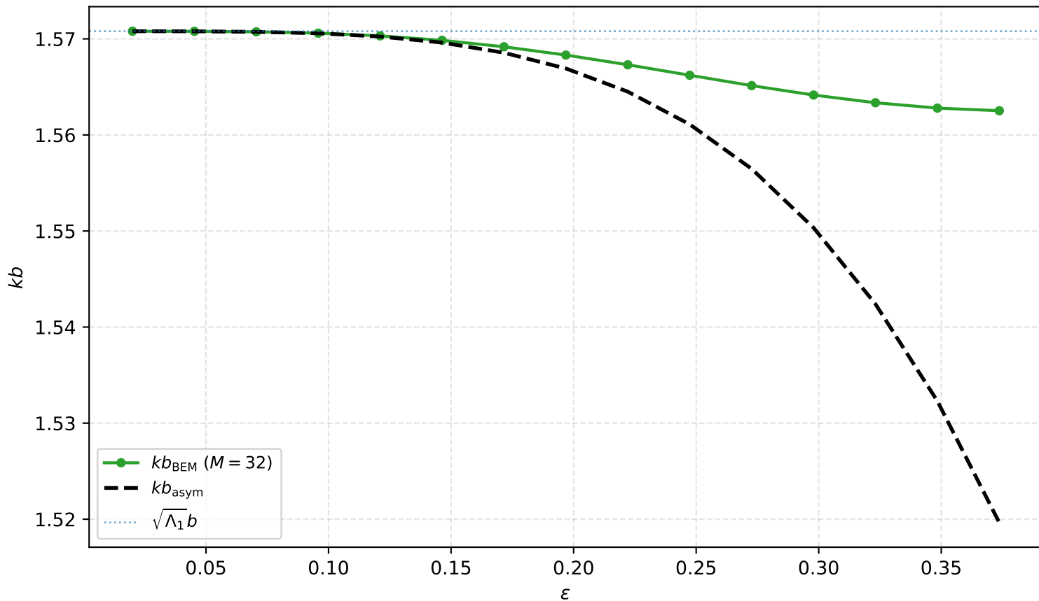
Theorem 2.1: kb versus \varepsilon , a = 0.55 , M = 32
