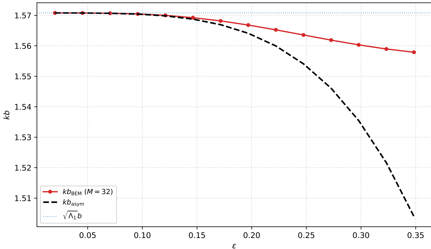
Theorem 2.1: kb versus \varepsilon , a = 0.60 , M = 32
