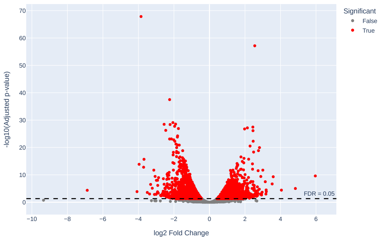
GSE263449_CAGE_nipbl2_deseq2_tpm0.5_results_uniq_22RV1: NIPBL KD vs Control (FDR &lt; 0.05)
