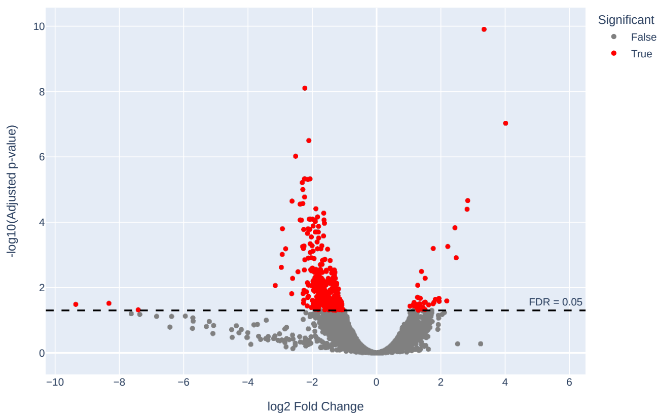
GSE263449_CAGE_nipbl2_deseq2_tpm0.5_results_uniq_VCAP: NIPBL KD vs Control (FDR &lt; 0.05)
