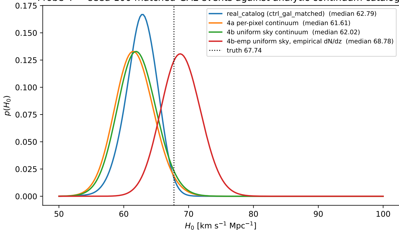
Probe 4 — seed-100 matched-GAL events against analytic continuum catalogs
