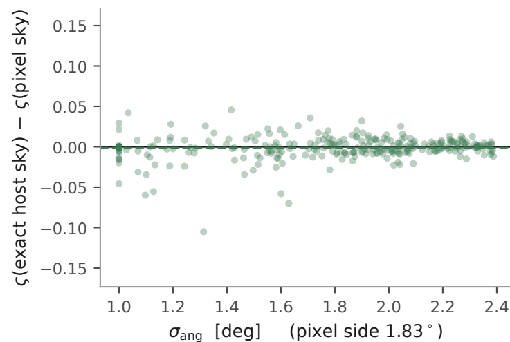
(b) the pixelisation term, per event mean -1.558\text{e-}03 \pm 9.0\text{e-}04
