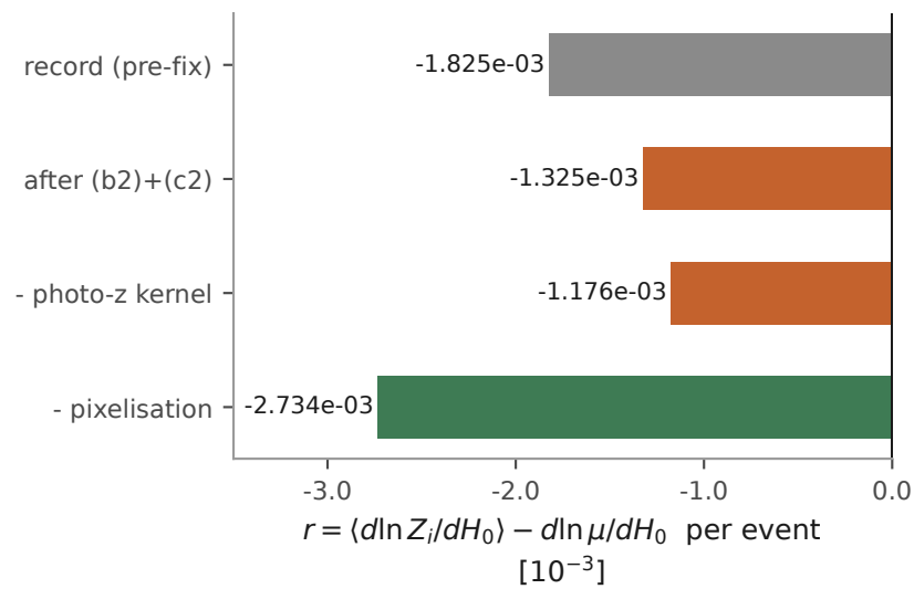
(c) the closure ladder
