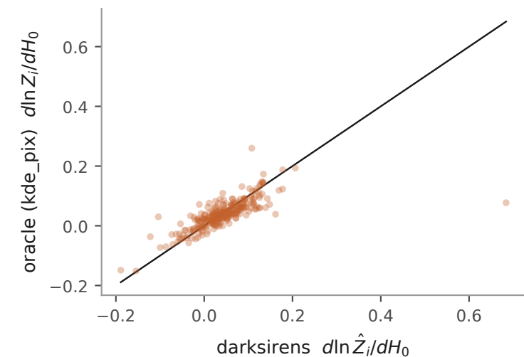
(a) anchor: -3.29\text{e-}03 \pm 2.8\text{e-}03 per event rms 4.698\text{e-}02 vs darksirens' own MC 3.165\text{e-}02
