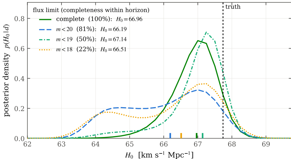
Anchored completeness ladder: H_0 posteriors (ticks: medians; common displacement = baseline bias)
