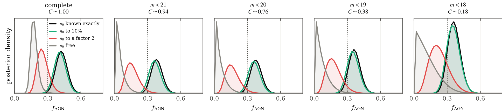
f_{\text{AGN}} recovery vs. density knowledge (dotted = planted value; exact/10% recover high, free recovers low)
