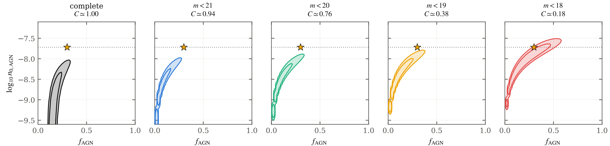
The (f_{\text{AGN}}, n_{0,\text{AGN}}) degeneracy (star = truth, dotted = true density)
