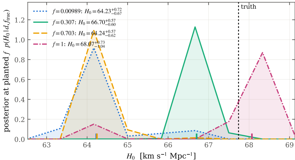
H_0 recovery at the planted AGN fraction, all four rungs: the tilt is non-monotonic in f_{\text{AGN}} (ticks: medians)
