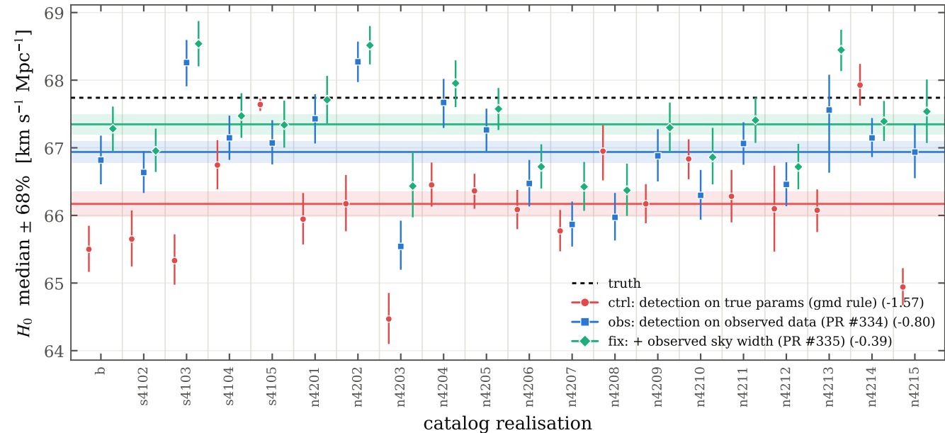
K=1 closure per realisation (arms paired by catalog; bands: arm mean \pm SEM)
