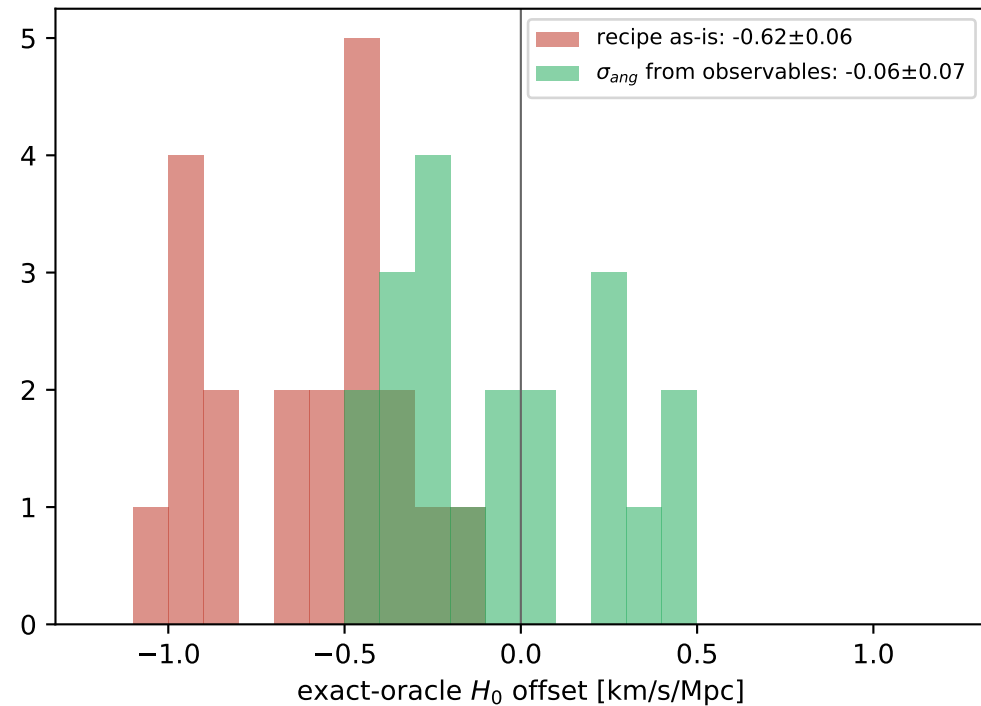
parametric bootstrap: latent sky width vs fix
