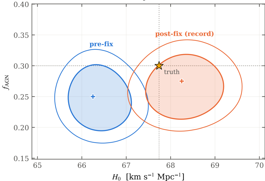
Joint 68/90% credible regions, N=200 (star + dotted cross = planted values, + = MAP)
