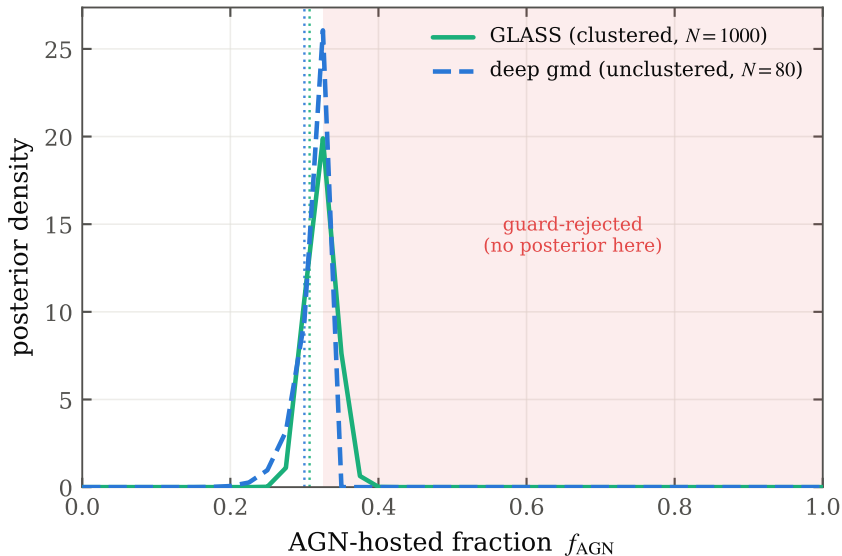
The AGN-hosted fraction on both mocks
