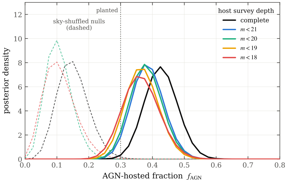
f_{\text{AGN}} recovery along the completeness ladder (post-fix)
