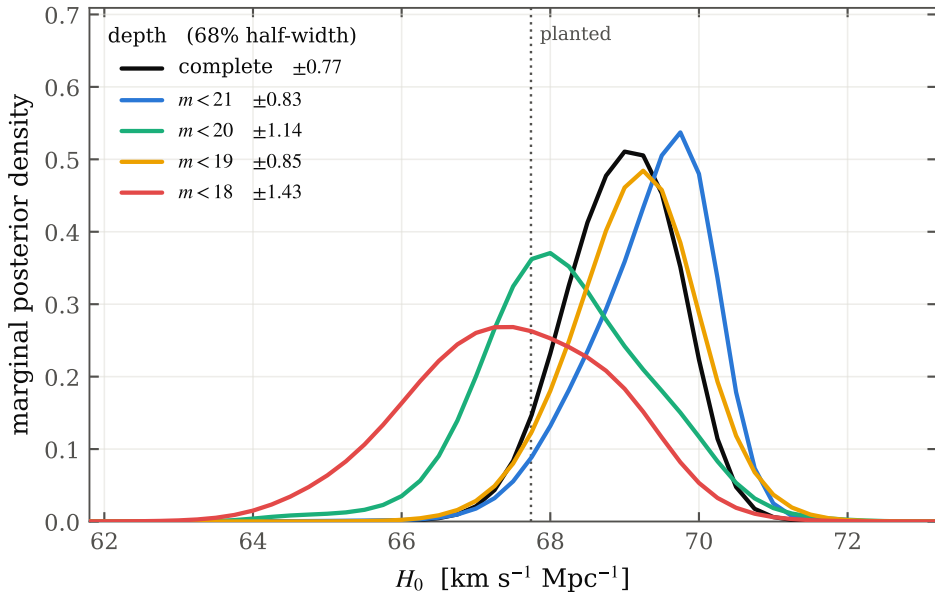
H_0 recovery along the completeness ladder (post-fix)
