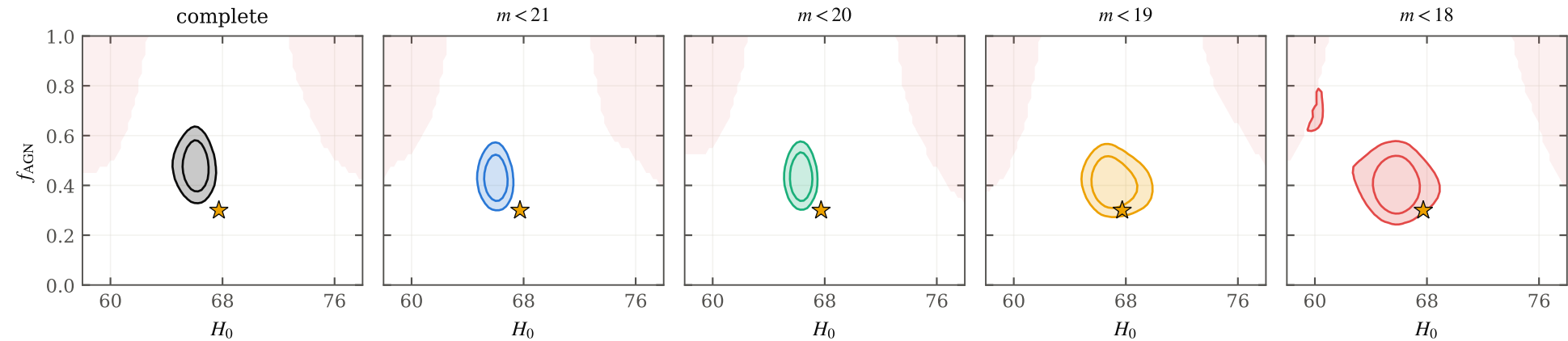
Two-tracer plane along the completeness ladder (star = truth, shaded red = inadmissible)
