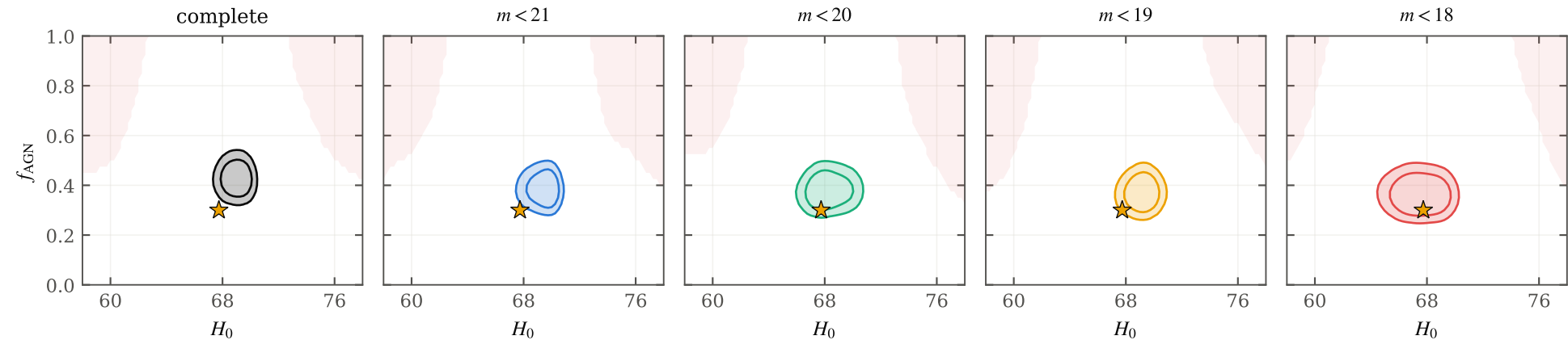
Two-tracer plane along the completeness ladder (star = truth, shaded red = inadmissible)
