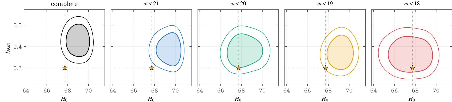
68/90% credible regions along the ladder (post-fix; star + dotted cross = planted values)
