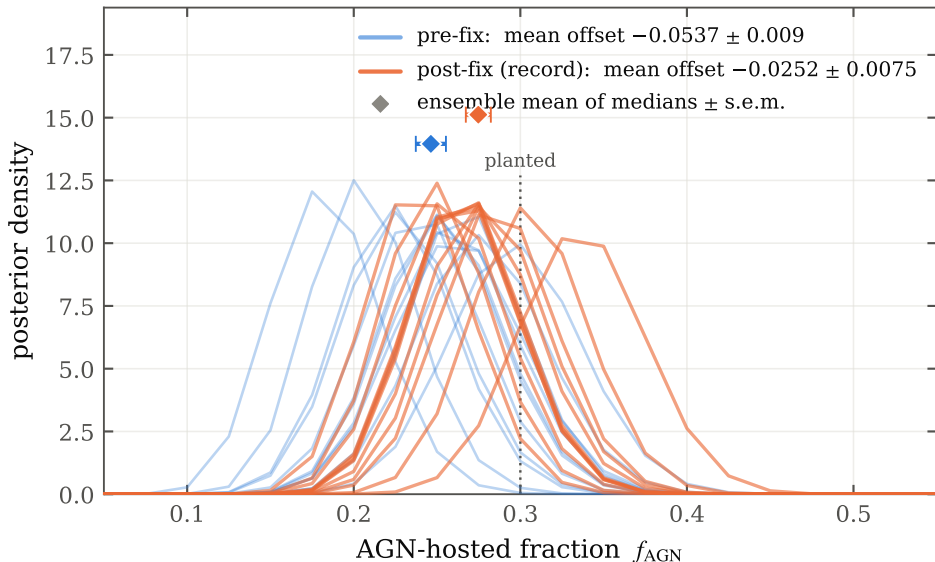
f_{\text{AGN}} recovery across 12 seeds, pre-fix vs \sigma_{\text{ang}} -fixed generator
