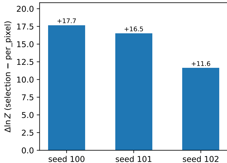
m<18 free anchors, darksirens 0c5b3db: the a5 headline replicates at three seeds
