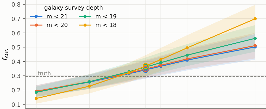
The completion's AGN density anchor sets the recovered AGN fraction
