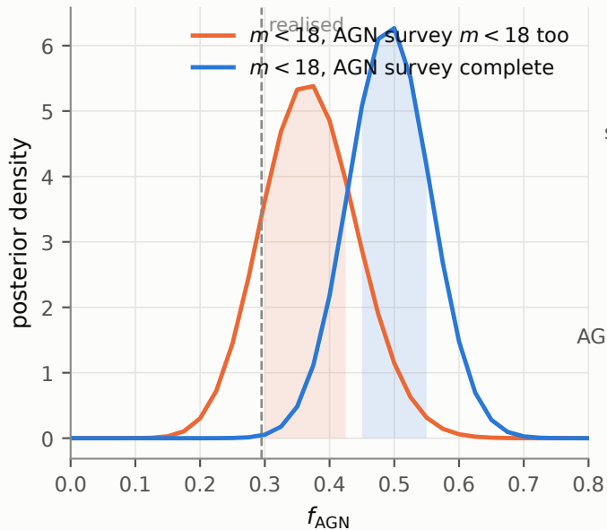
Faintest rung, AGN completion removed
