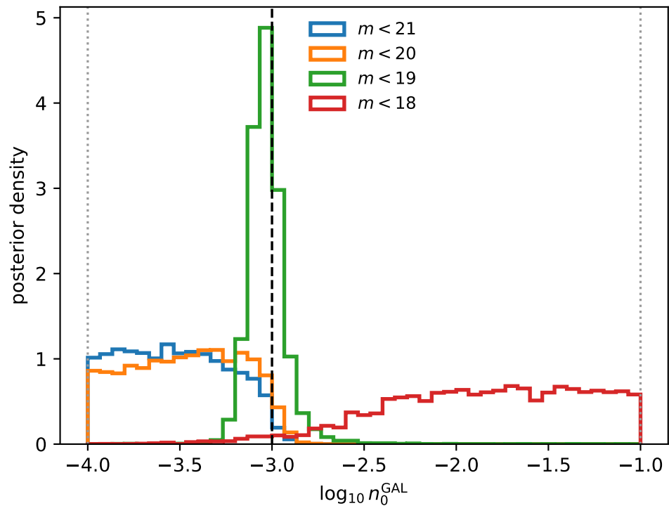
Galaxy anchor: recovered at m < 19 , railed at m < 18
