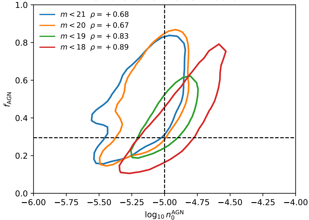
AGN anchor vs. the AGN fraction
