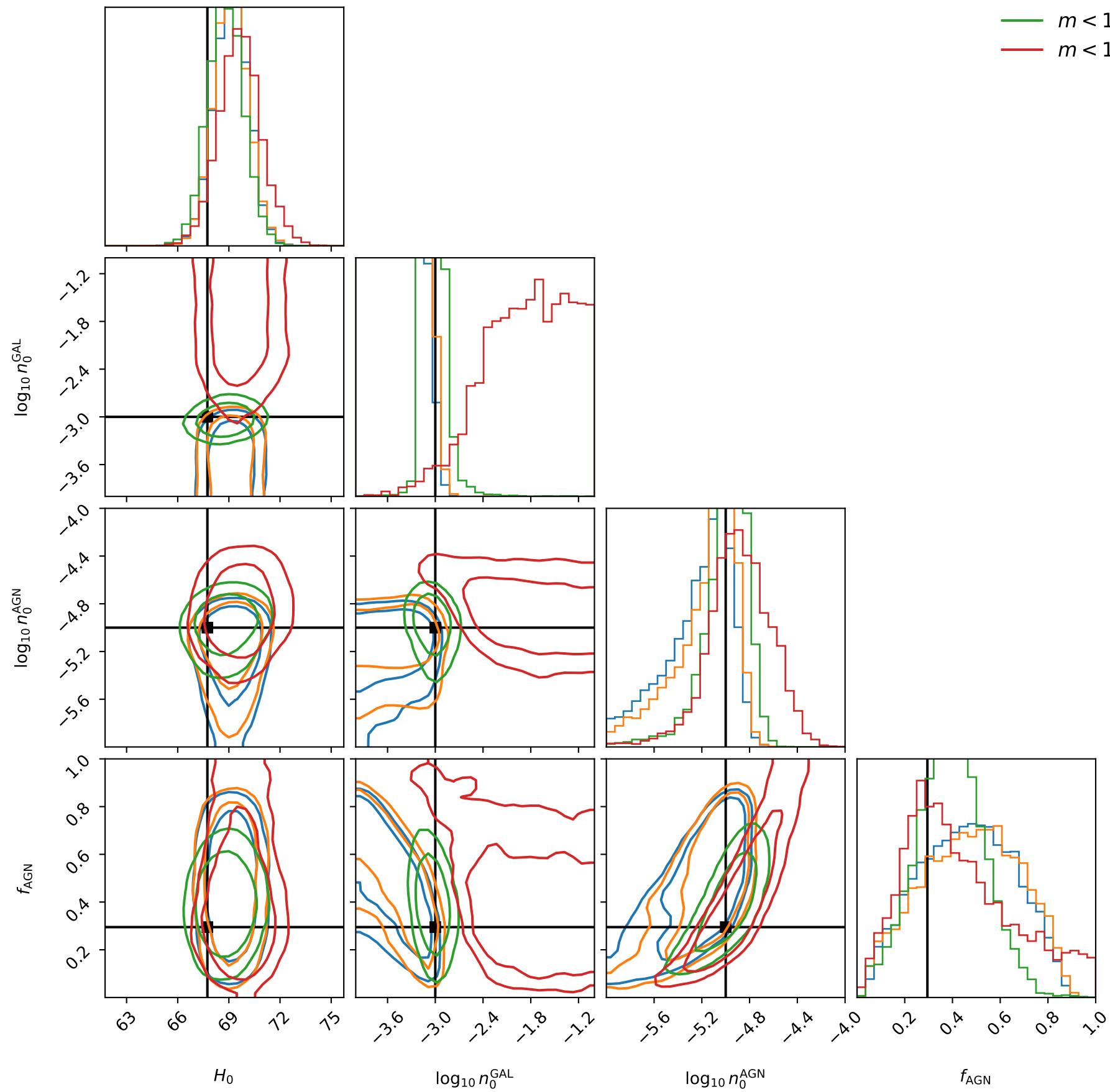
Four free parameters down the ladder (dynesty, nlive 1000)
