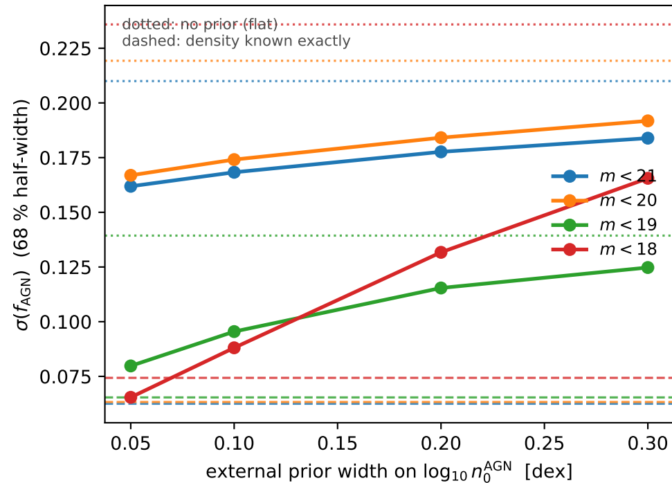
the width shrinks...
