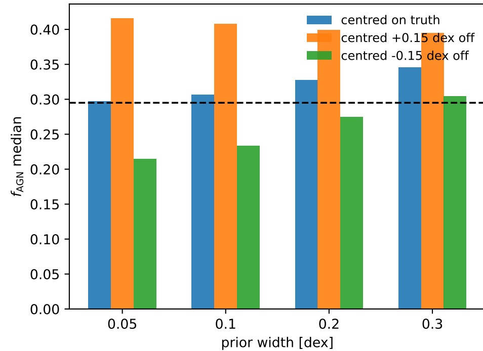
m < 18 : a wrong prior is worse than none
