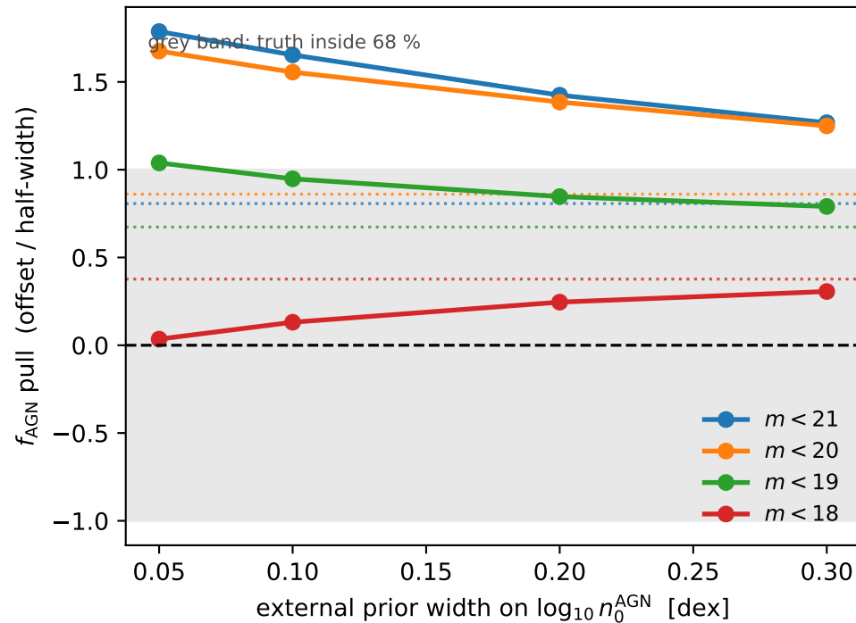
...but only m < 19 and m < 18 stay honest
