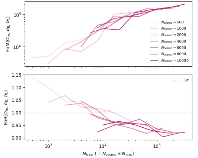
Figure 10. Convergence of the inference with training set size, for P_{\text{gg}}(k) + B_{\text{ggg}}(k_1, k_2, k_3) + P_{\text{gm}}(k) on the coverage test set for the three key parameters \Omega_m , \sigma_8 , and b_1 combined. The top panel shows the figure of merit (FoM), and the bottom panel shows the figure of bias (FoB), normalized by the 68th percentile of the \chi^2 distribution for three dimensions (corresponding to the three parameters); the median values over the coverage set are shown. The opacity indicates the number of training cosmologies. Increasing the number of training points increases the precision significantly until N_{\text{train}} \sim 20,000 and then more marginally, with the number of cosmologies and bias parameter sets contributing similar precision; the bias also plateaus around N_{\text{train}} \sim 20,000 , with the number of cosmologies mattering more than the number of bias parameters for smaller N_{\text{train}} . ksf: make legends, axis labels bigger ksf: note: this plot is with an older base model, with kmax=0.4 and no ensembling; running the new version right now
