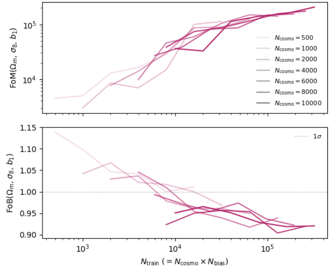
Figure 10. Convergence of the inference with training set size, for P_{\text{gg}}(k) + B_{\text{ggg}}(k_1, k_2, k_3) + P_{\text{gm}}(k) on the coverage test set for the three key parameters \Omega_m , \sigma_8 , and b_1 combined. The top panel shows the figure of merit (FoM), and the bottom panel shows the figure of bias (FoB), normalized by the 68th percentile of the \chi^2 distribution for three dimensions (corresponding to the three parameters); the median values over the coverage set are shown. The opacity indicates the number of training cosmologies. Increasing the number of training points increases the precision significantly until N_{\text{train}} \sim 20,000 and then more marginally, with the number of cosmologies and bias parameter sets contributing similar precision; the bias also plateaus around N_{\text{train}} \sim 20,000 , with the number of cosmologies mattering more than the number of bias parameters for smaller N_{\text{train}} . ksf: make legends, axis labels bigger ksf: note: this plot is with an older base model, with kmax=0.4 and no ensembling; running the new version right now
