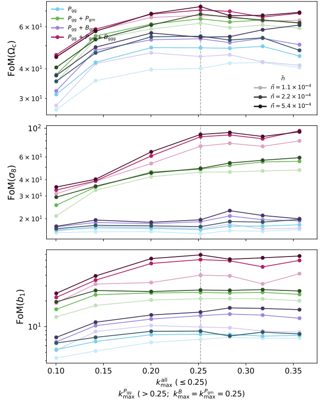
Figure 9. Scale dependence of the figure of merit (FoM) for the three key parameters for the SHAMe out-of-distribution mock, with varying number density. The k_{\max} displayed is defined as follows: for k_{\max} < 0.25 , k_{\max} = k_{\max}^{P_{gg}} = k_{\max}^{P_{gm}} = k_{\max}^{B_{ggg}} ; for k_{\max} > 0.25 , we fix k_{\max}^{P_{gm}} = k_{\max}^{B_{ggg}} = 0.25 and only vary k_{\max} = k_{\max}^{P_{gg}} . Precision generally increases with scale, especially from k_{\max} = 0.1 to k_{\max} = 0.25 , with additional gains for \sigma_8 when extending to k_{\max}^{P_{gg}} = 0.37 . ksf: make legends, axis labels bigger
